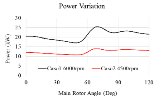
Figure 7. Compression power variation during a cycle
