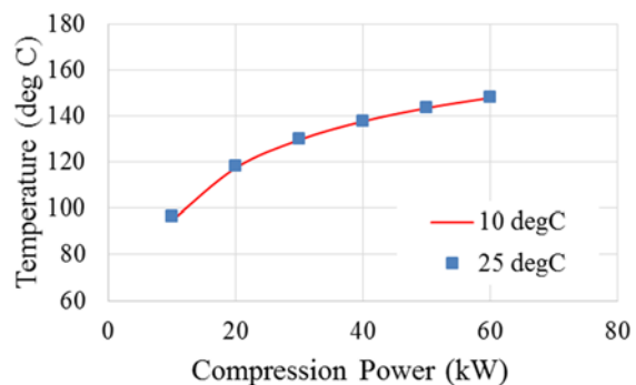
Figure 3. Saturation temperature of air at 11.0 bar discharge
