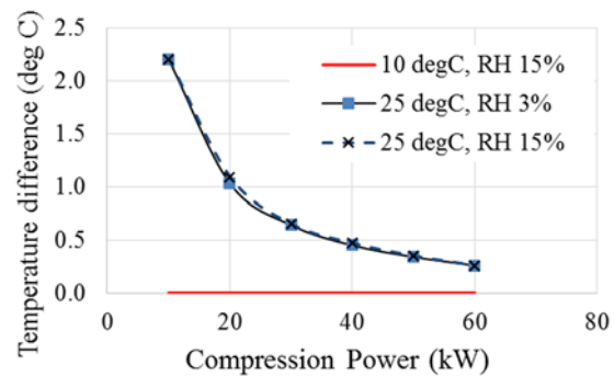
Figure 5. Delivery temperature variation relative to 3% RH
