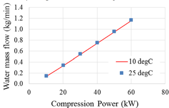
Figure 2. Water mass flow required for saturation of air at 11.0 bar discharge
