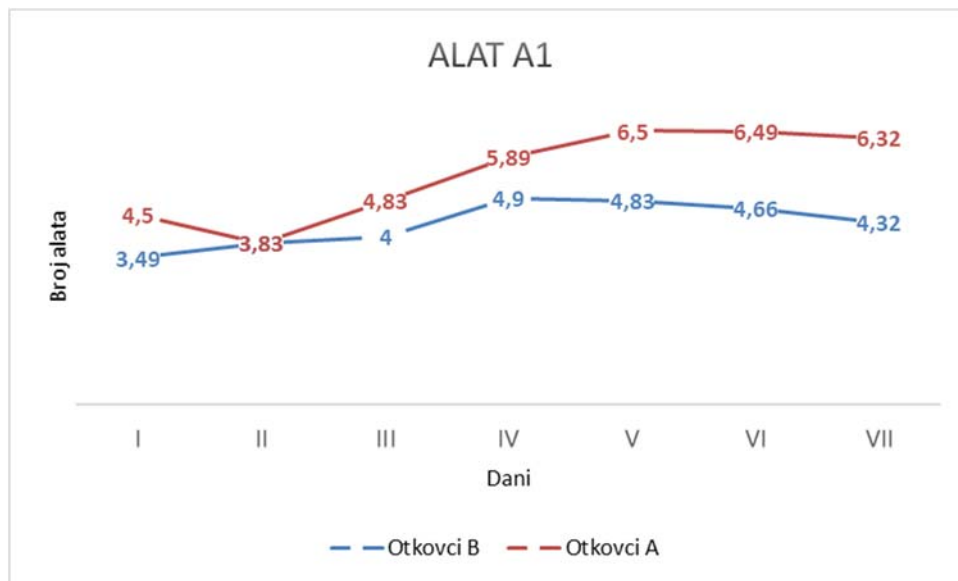
Grafikon 1. Prikaz dnevne potrošnje alata A1 za obradu otkovaka Chart 1. Displaying the daily consumption of the A1 tool for processing forgings
