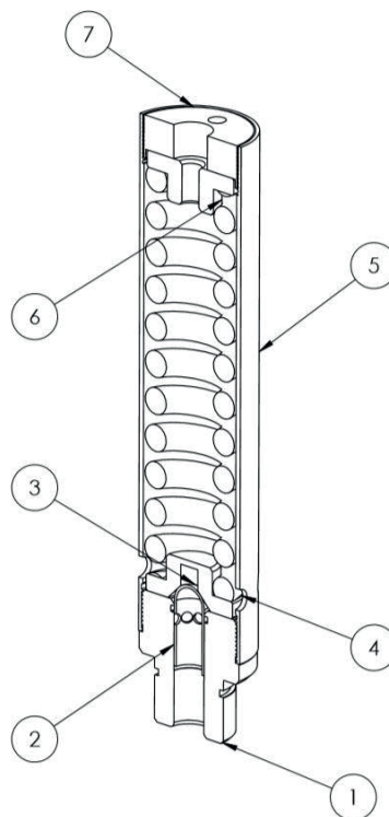
Figure 3 Piston valve assembly cross section
