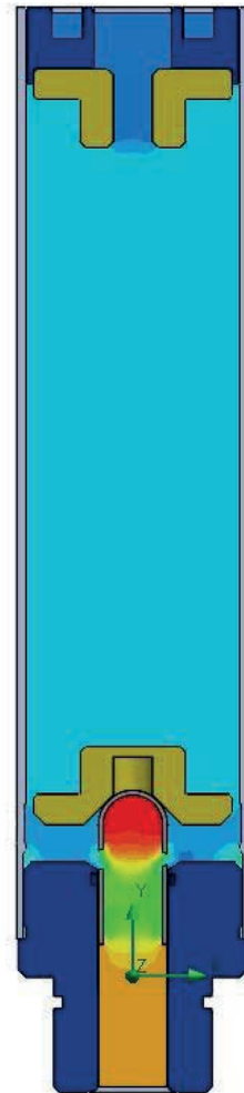
Figure 11 Pressure distribution in valve
