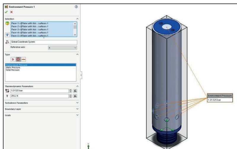
Figure 9 Boundary conditions
