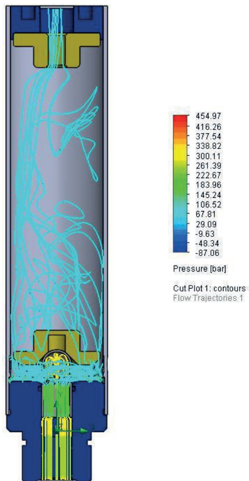
Figure 10 Fluid flow trajectories
