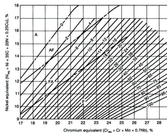
Figure 8 WRC-1992 diagram [9,13]
