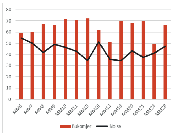
Figure 10 The difference between the results of the measurement by sound level meter and the results obtained by calculation in iNoise
